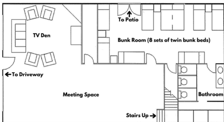
Downstairs
